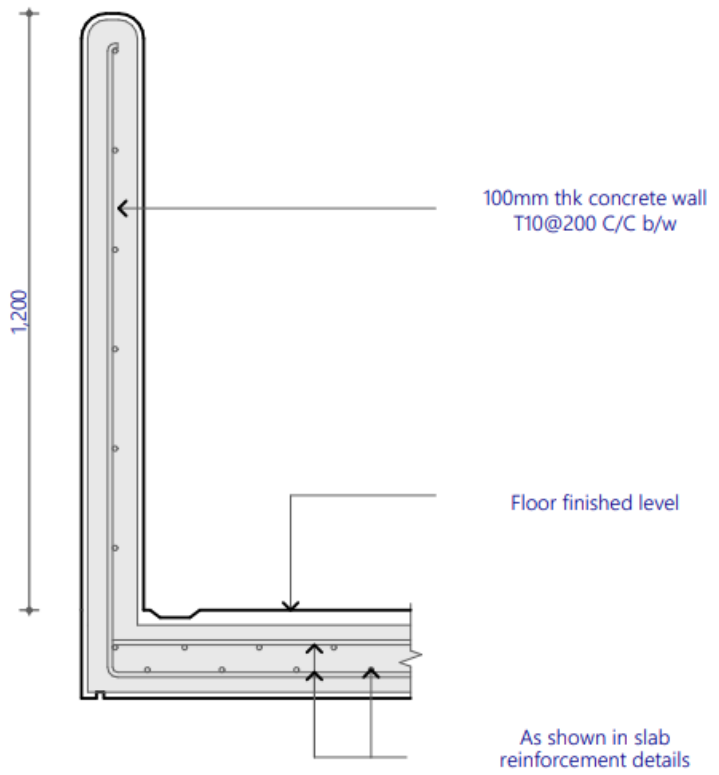
Sectional View
